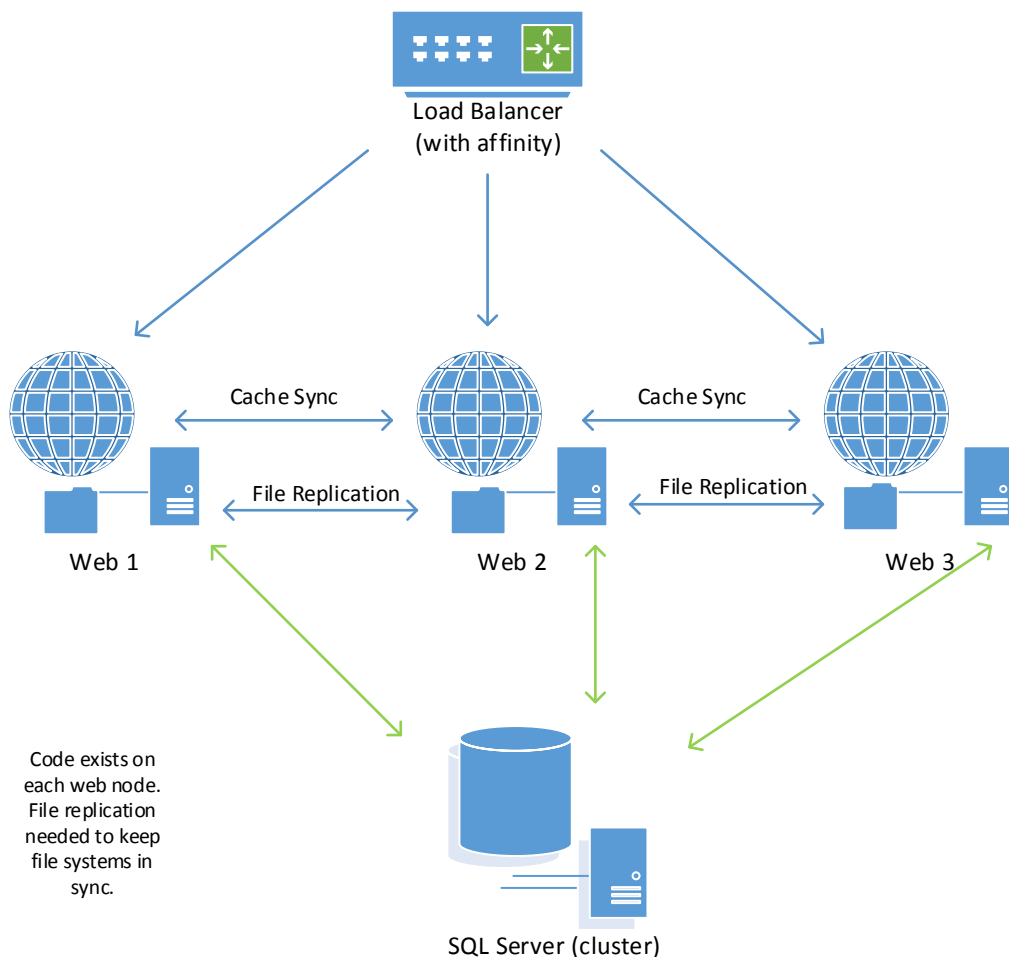
Figure 3 – File Replication
